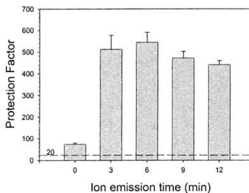
Figure 3. Protection factor of R95 respirator enhanced by VI-2500 (averaged over d_p=0.04-0.20 \mu\text{m} ).
