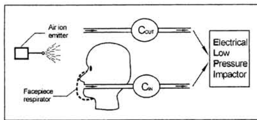
Figure 1. Experimental set-up.
