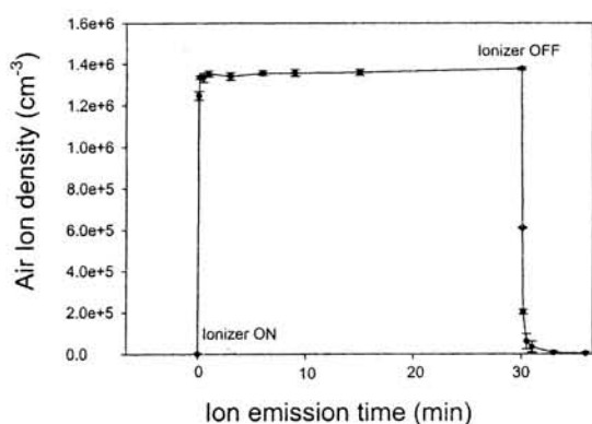
Figure 2. Air ion density as a function of time during unipolar ion emission by VI-2500 in the chamber.
